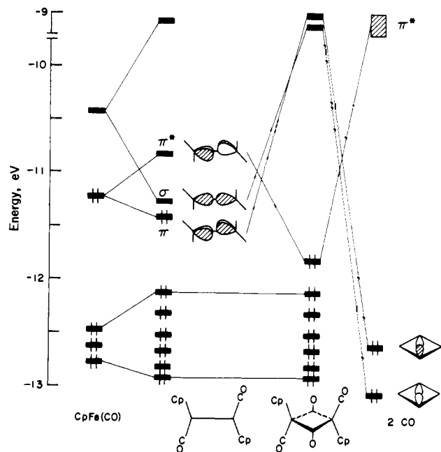
Figure 3. Interaction diagram for the formation of trans -Cp 2 Fe 2 (CO) 2 from two CpFeCO, and for trans -Cp 2 Fe 2 (CO) 4 from Cp 2 Fe 2 (CO) 2 and two CO's.
